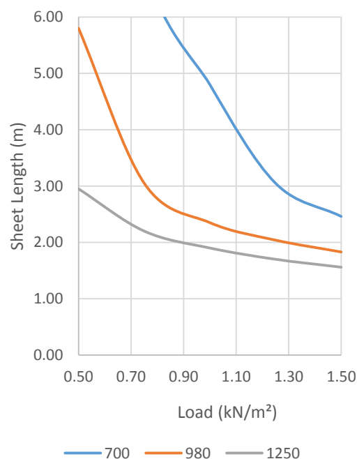
Load/Span
